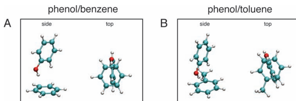
Figure 2. Geometry-optimized structures of the (A) phenol/benzene and (B) phenol/toluene complexes are shown in side and top views.
